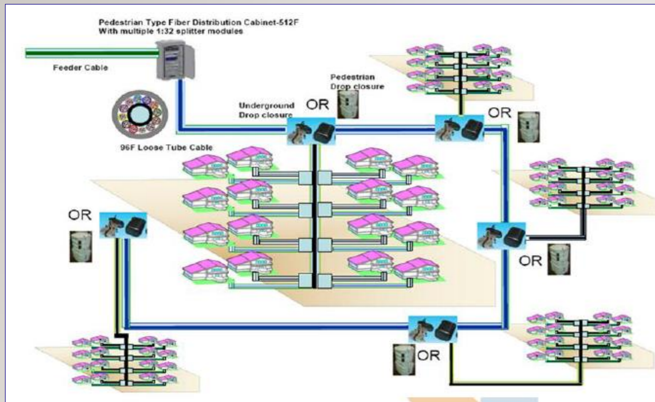
a) One Stage Passive Splitter
