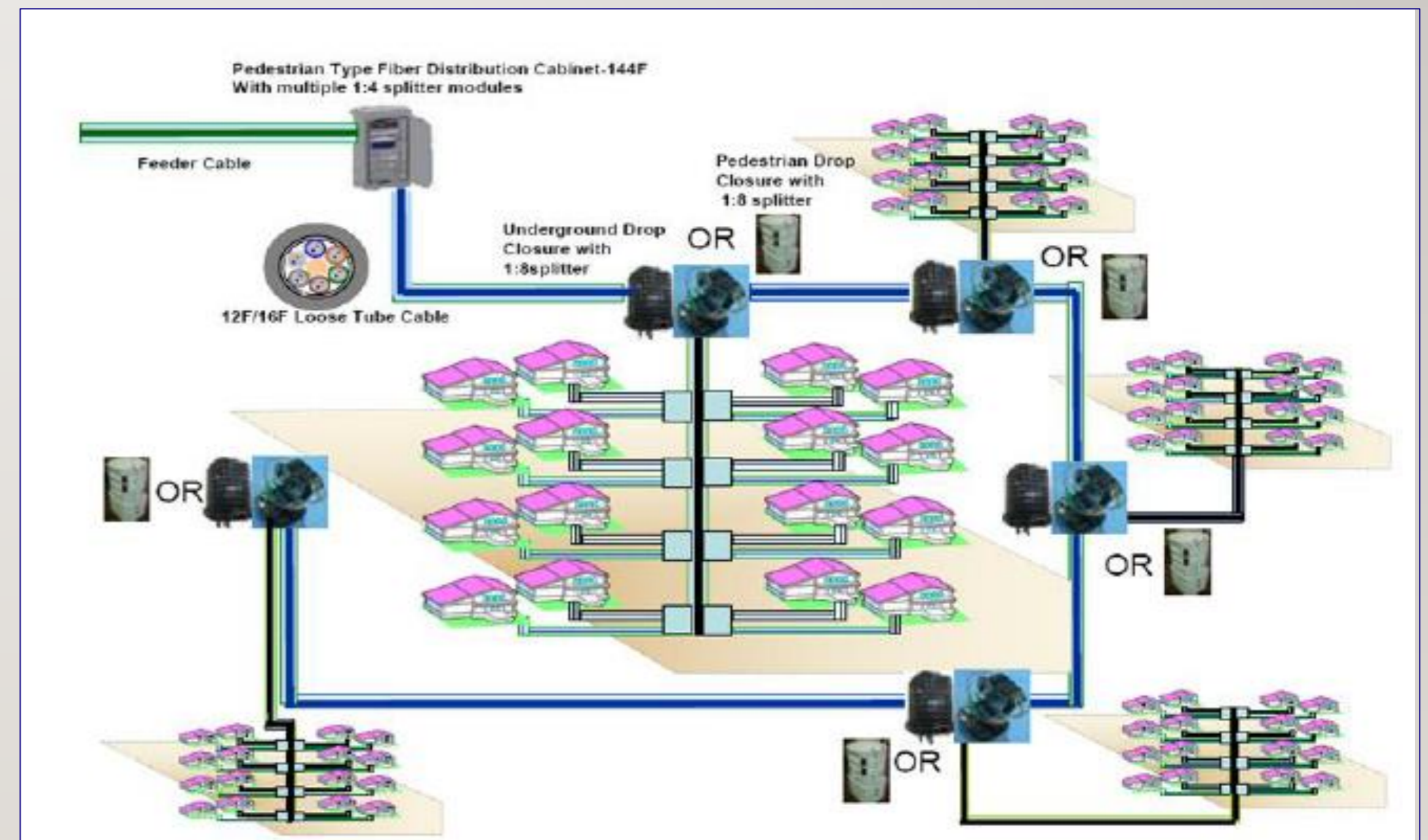
b) Two Stage Passive Splitter
