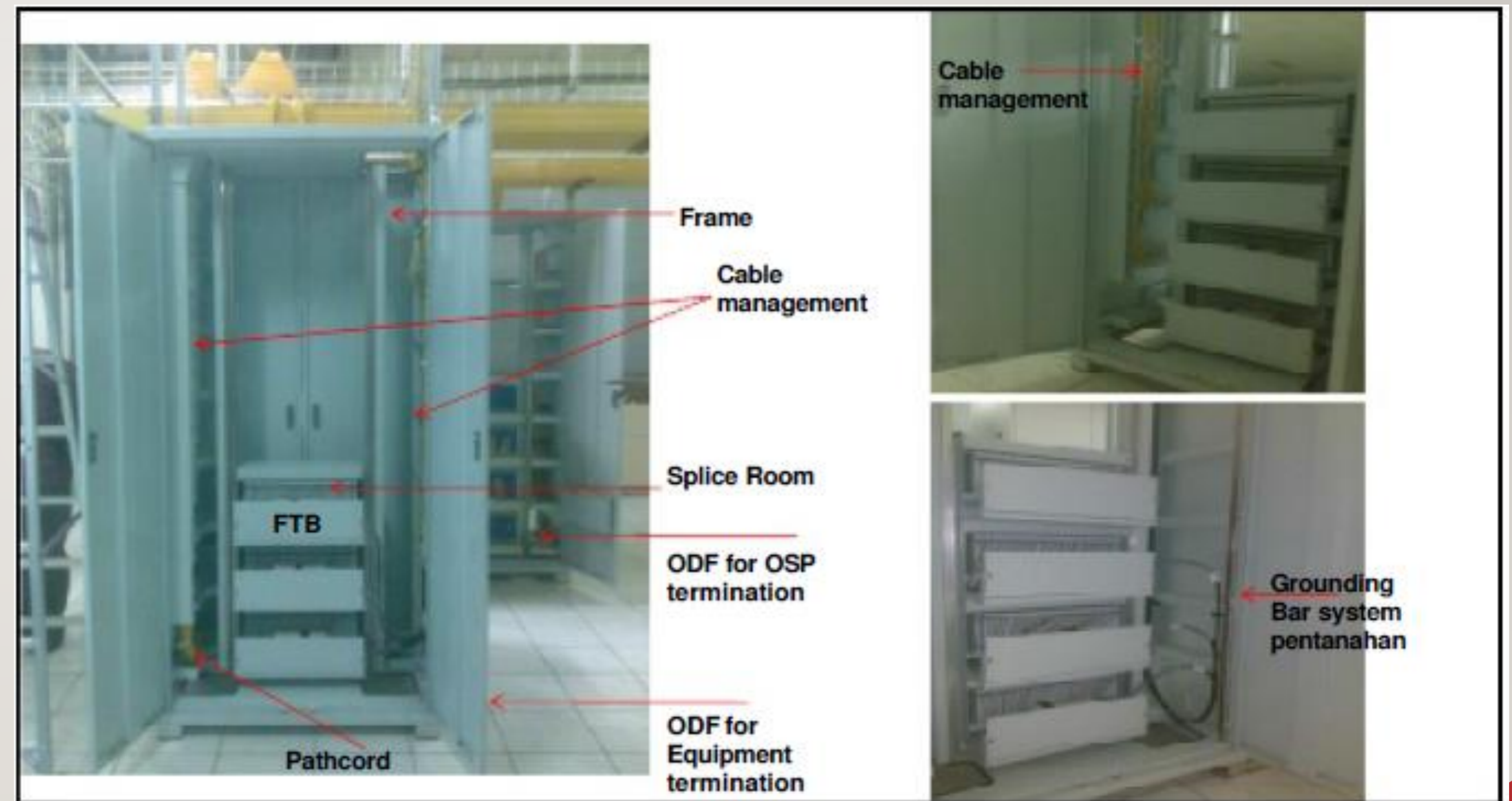
Gambar. ODF ( Optical Distribution Frame)
